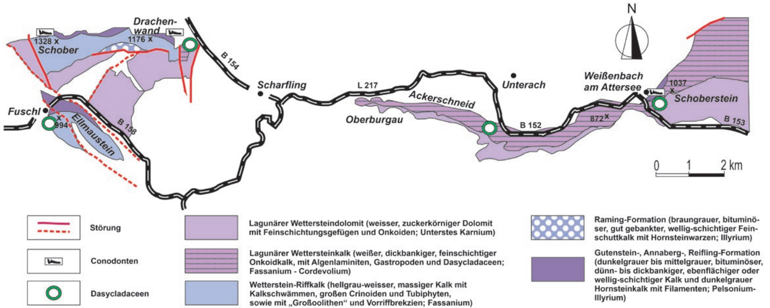
ABB. 3: Geologie der Mitteltrias zwischen Fuschlsee und Attersee FIG. 3: Geology of the Middle Triassic stratigraphic units between the lake Fuschlsee and the lake Attersee (Upper Austria)
